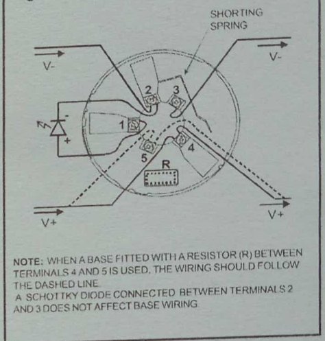
Figure 1: Base Terminal Wiring
